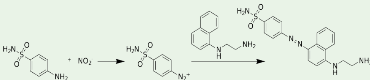
Figure 1: Illustration of the Griess Test Reaction.
