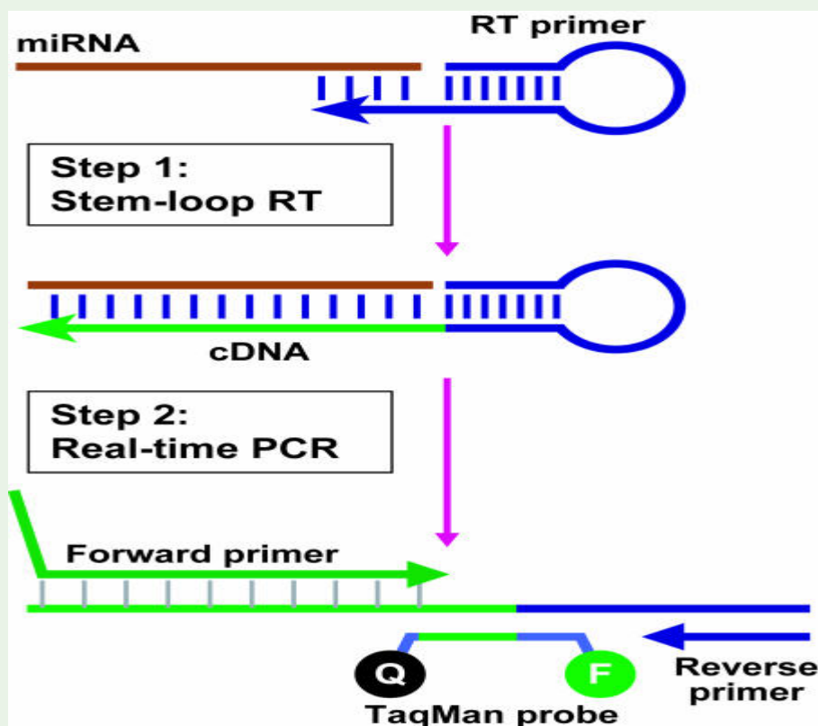
Figure 3: Real-time quantification of microRNA by Stem-loop RT-PCR [68].
